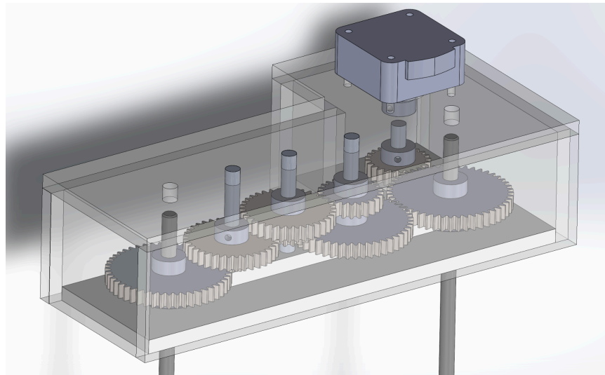
Fig. 26: Final SOLIDWORKS model for the gearbox and gear train (created by authors).
