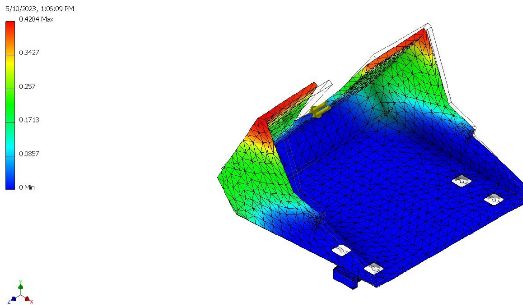
Figure 18: Nexsteer Mount FEA Deformation Results. (Cameron Chiaramonte, 2023)
