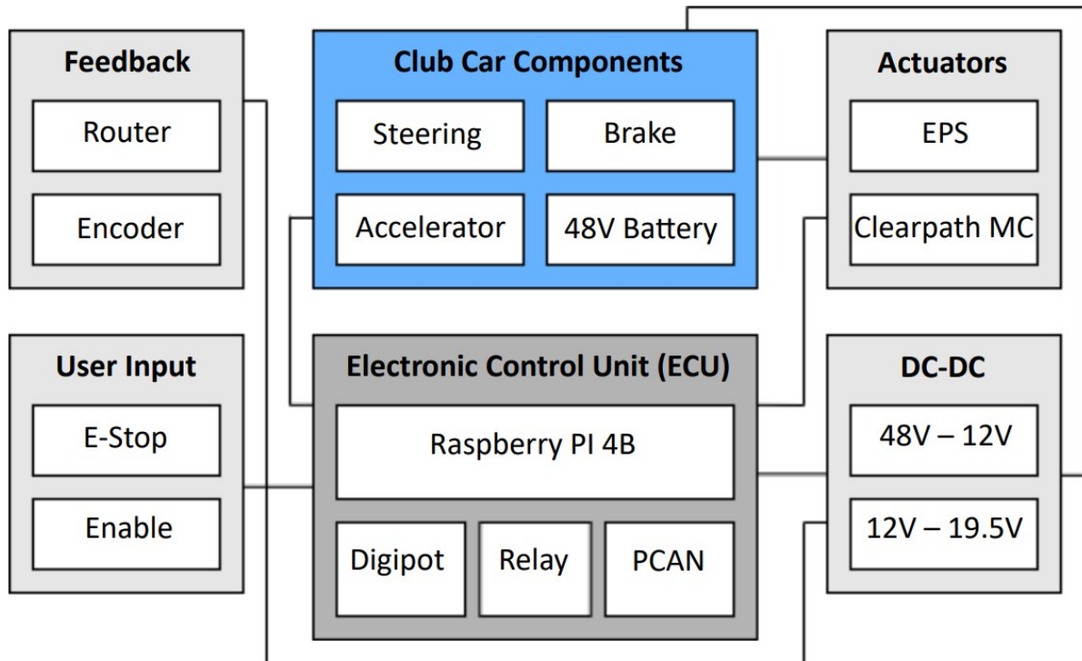
Figure 5: Overview of Final System Components. (Gilchrist Johnson, 2023)
