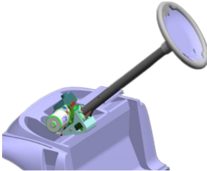
Figure 6: CAD Model of Nexteer Electric Power Steering Module. (Credit: Furukawa et al., 2018)
