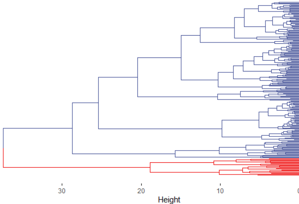
Fig. 4: Full Dendrogram
