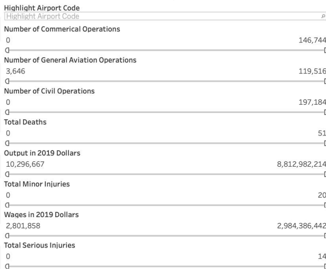
Fig. 8: Interface Design
