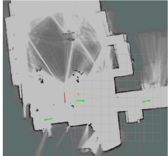
Fig. 4: Waypoint markers (green) within a 2-dimensional map of the arena created by Cartographer's SLAM algorithm with LiDAR input.
