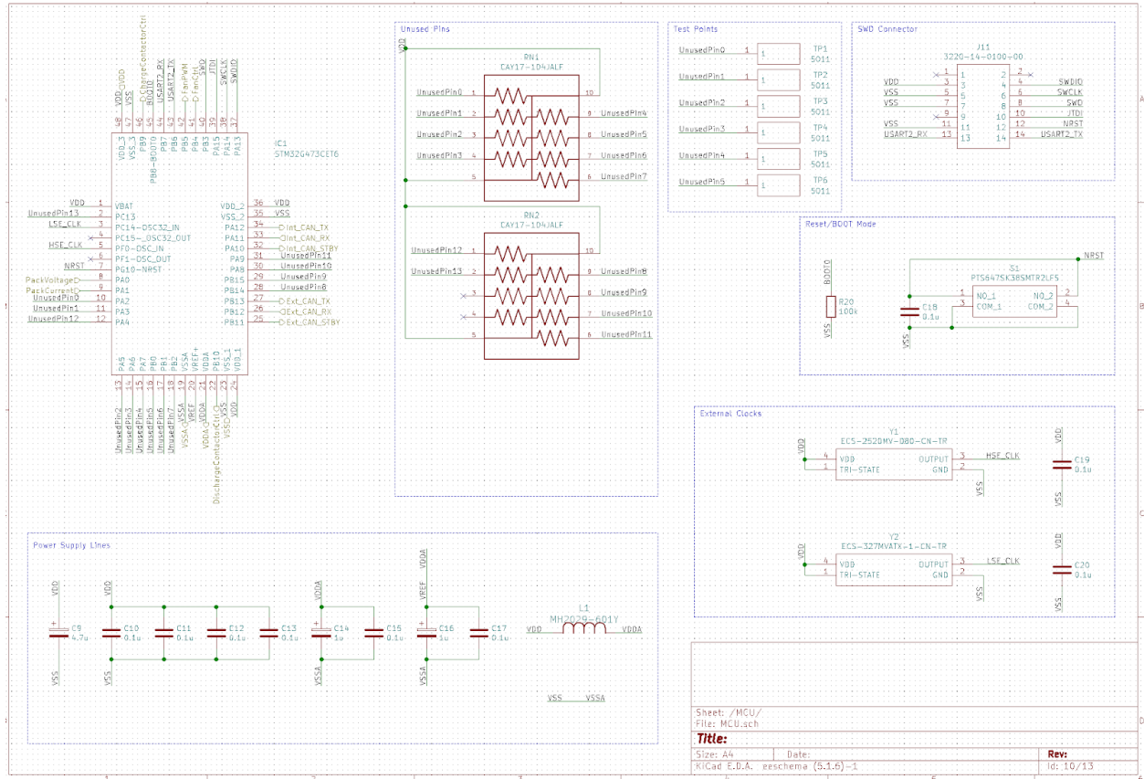
Figure 4. Main Node MCU Schematic
