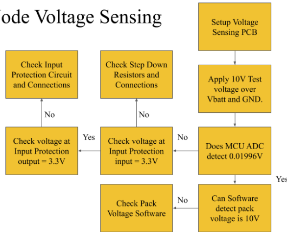
Figure 40. Main Node Voltage Sensing Test Plan
