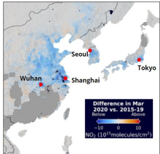
Fig. 2. Differences in \text{NO}_2 in the Asia-Pacific Region
