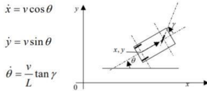
Figure 11: Equations of motion for Ackerman steering vehicles. x, y, and theta represent the vehicle's position and orientation in the global frame and v and gamma represent the control inputs of speed and steering angle, respectively. L is the distance between the front and back wheels.
