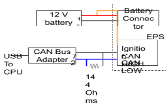
Figure 14: Circuit diagram for CAN communication
