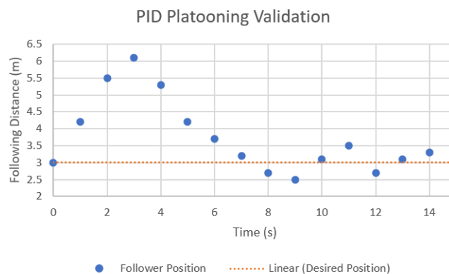
Figure 31: PID Platooning Validation
