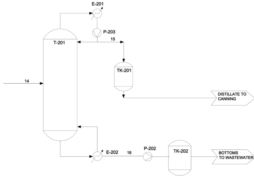
Figure 2. Distillation Block Flow Diagram
