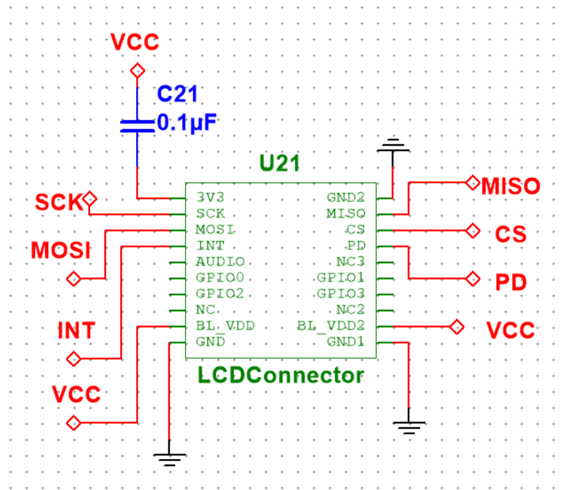
Figure 10: Connections to the LCD TFT Display
