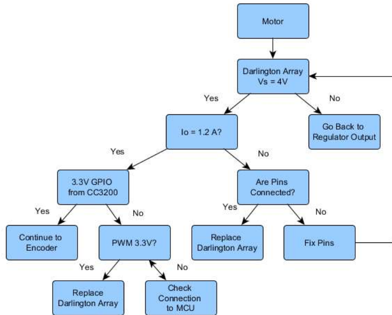
Figure 24:Motor Test Plan
