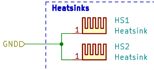
Figure 31: Heatsink schematic
