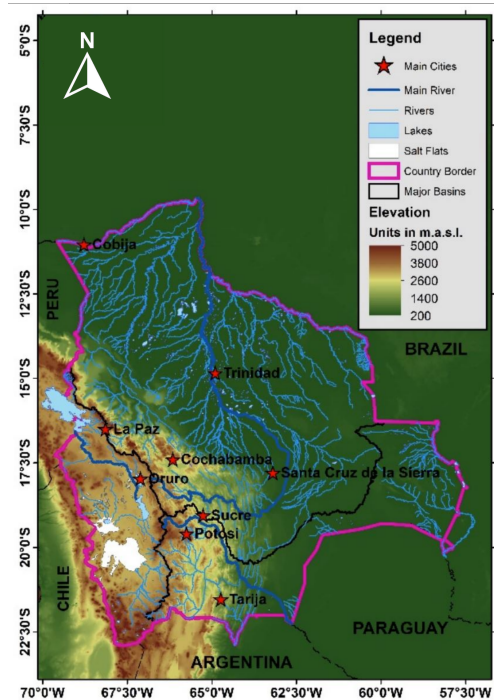
Figure 3.5.4. Hydrological Map of Bolivia (Saavedra et. al., 2022).
