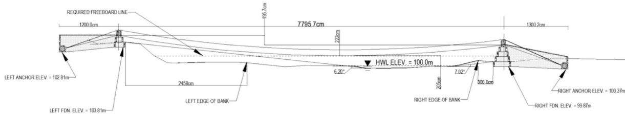
Figure 4.4.1. Design #2 Standard Geometric Layout.
