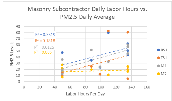
Figure 2. Subcontractor presence vs. PM2.5 daily average across site
