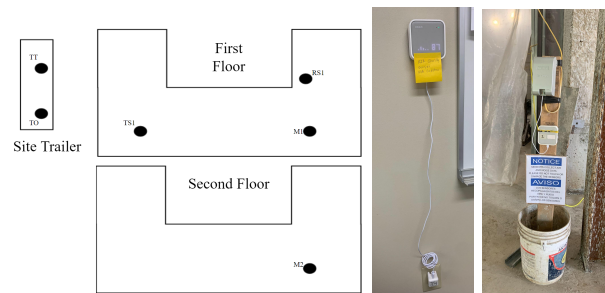
Figure 1. On-site sensor locations
