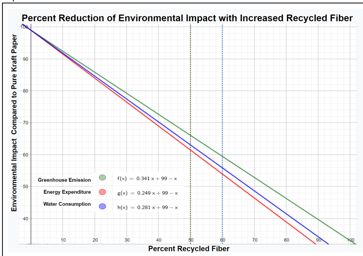
Figure 18: showing the reduction of greenhouse emission, energy expenditure, and water consumption based on the percentage increase of recycled fiber content per ton of paper. Y-intercept displays baseline environmental impact of a 100% Kraft pulp paper. Units for greenhouse emission are in Kg of CO 2 equivalence per ton, units for energy expenditure are in kWh per ton, units for water consumption are in liters per ton. Vertical lines at 50% and 60% demonstrate visually the modest 10% increase in recycled fiber can have across these three LCA values. Note that 2% of the fiber is BNC and environmental impacts related to its processing are not shown.
