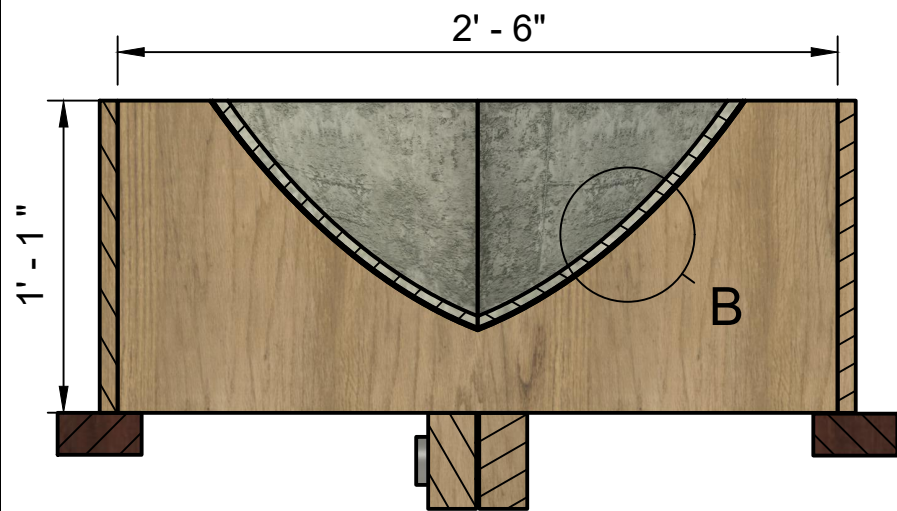
Section A - A Scale 1:8
