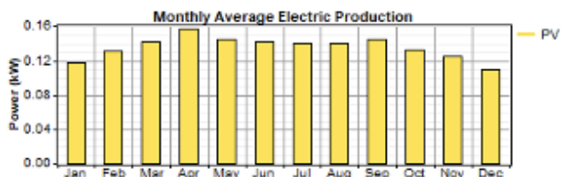
Fig. 3. Monthly Average Electric Production
