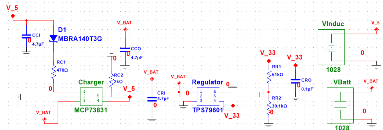
Figure 3 Power Schematic
