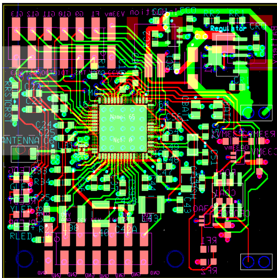
Figure 7 Second Board Layout
