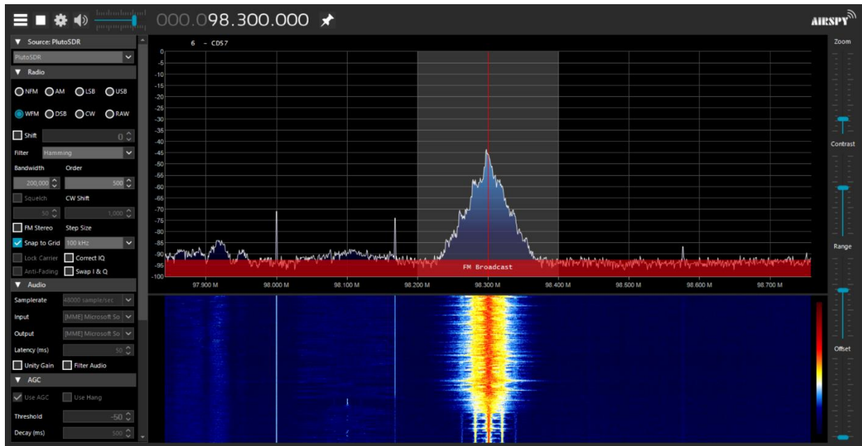
Figure 16: Signal Transmission
