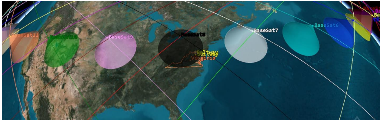
Figure 5. Constellation ground trace of CLAYTON's satellites with estimated imager range. The colored lines represent the multiple paths of the satellites. Each satellite is equipped with an imager, and the range the imager can view is pictured with the colored cone.
