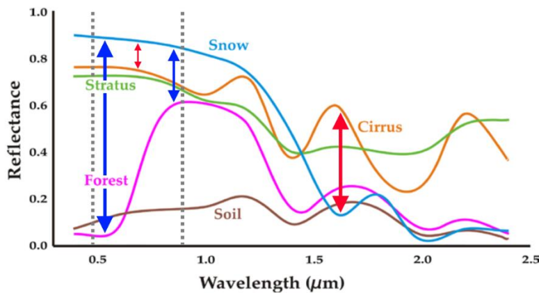
Figure 2.1 – Spectral reflectance of natural surfaces and clouds
