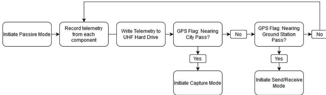
Figure 11: Passive Mode
