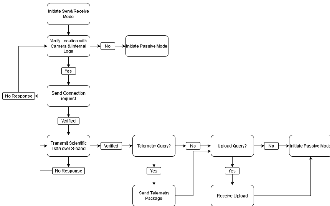
Figure 13: Send/Receive Mode
