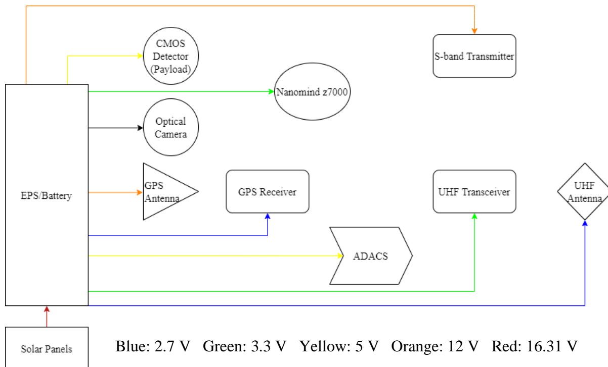
Figure 5: Power Flowchart
