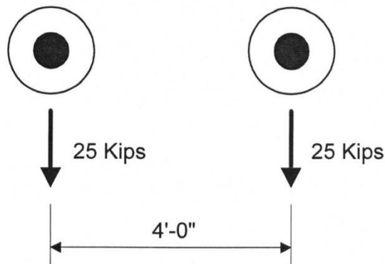
Figure 16: AASHTO design tandem wheel sideview to illustrate the axle spacings and axle loadings.
