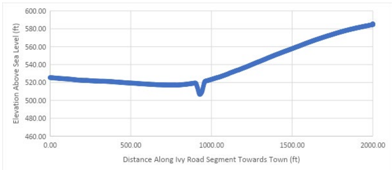
Figure 13: Graph showing distance along roadway versus the elevation above sea level. This is for the entire segment shown above.
