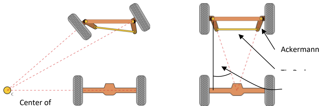
Figure 3. Variable wheel turning radius when rounding a turn
