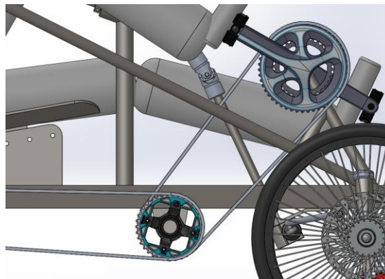
Figure 7. Crankshaft and two-chain assembly junction point for the drivetrain. Some parts are not finalized in the model, but the sizing is accurate.
