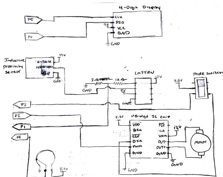
The coil counter is run by a Propellor 2 chip, and its wiring can be found below.
