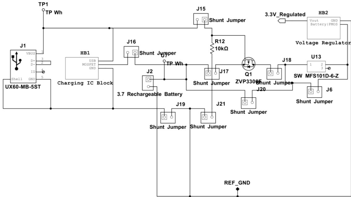
Figure 5: Power Unit Topology
