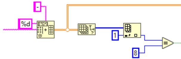
Figure 26: Data Verification
