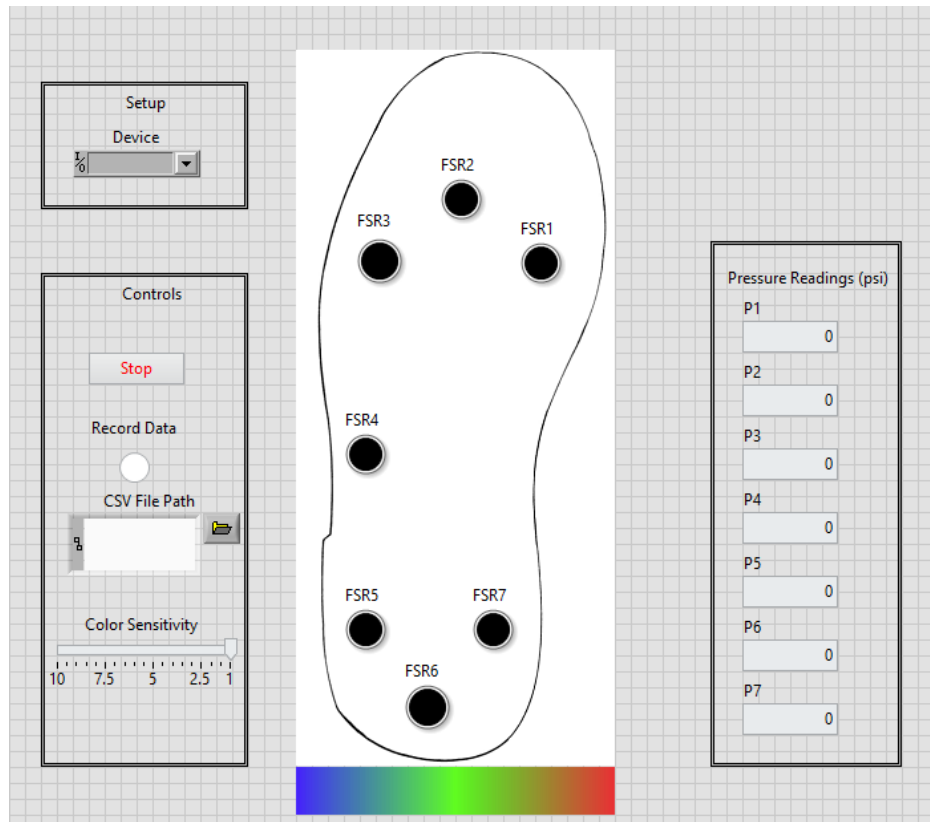
Figure 21: User Interface
