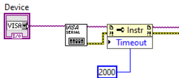
Figure 23: Connection Initialization
