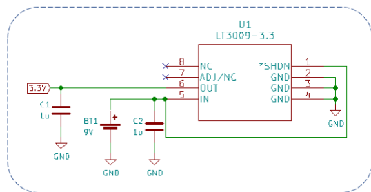
Figure 1: 3.3V Regulator
