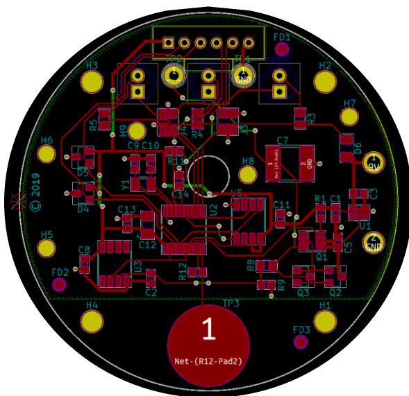
Figure 10: Device Layout
