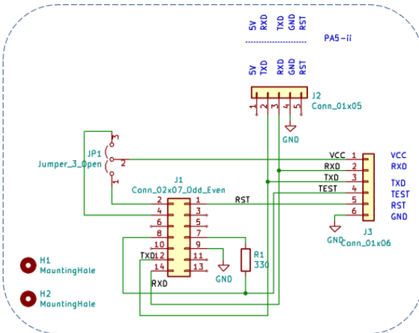
Figure 9: Adapter Board
