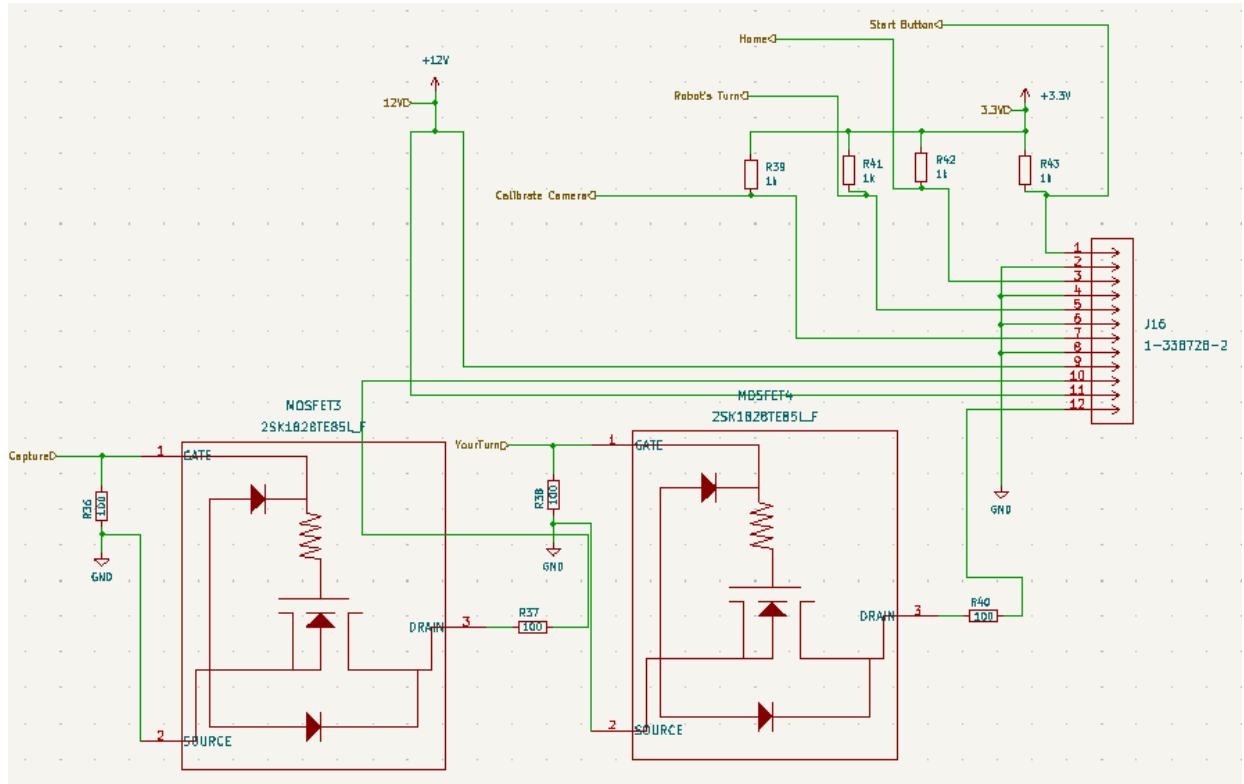
Figure 16: User Interface Panel Schematic
