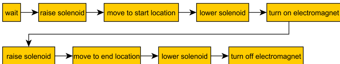
Figure 7: FSM Sketch
