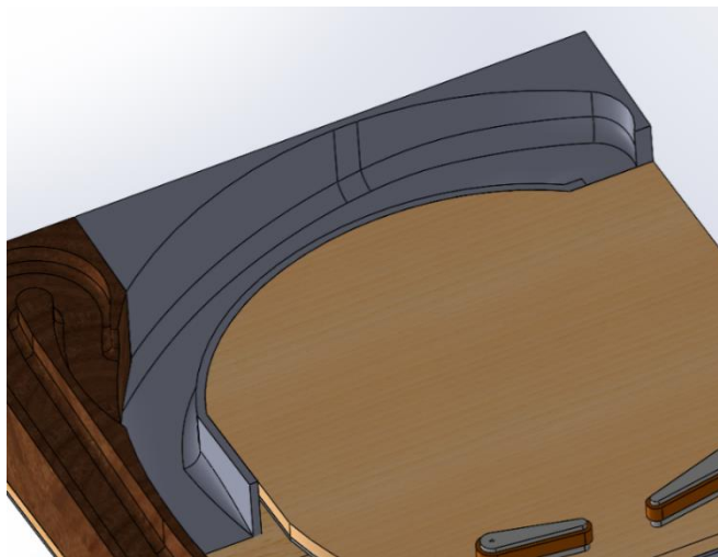
Fig. 3.3.1. Upper Playfield Ramp in Assembly
