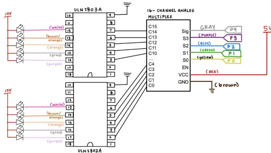
Fig. 2.1.11. Custom light control board with two Darlington transistor arrays, and 16-channel analog multiplexer.
