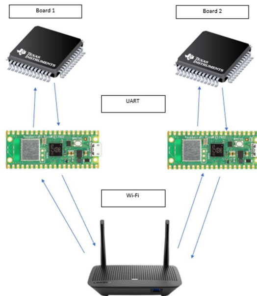
Figure 16 Communication Sequence
