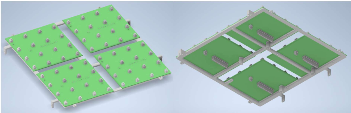
Figure 6 Button PCBs on Main Frame from Above and Below
