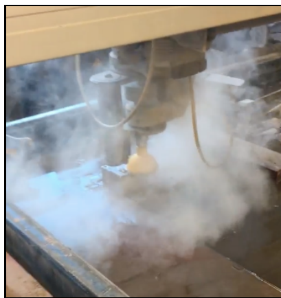
Figure 5. Waterjet Blasting into an Aluminum Block.
