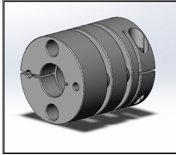
Figure 7. 3D Model of the ½” x 10mm Coupler for the PM-727V.
