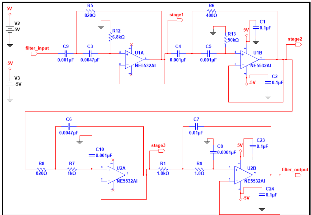
Figure 2: Filter Design
