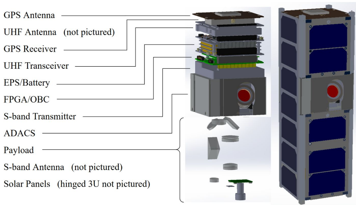
Figure 14: System Assembly
