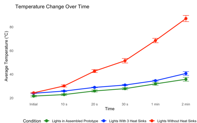
Figure 4. Results of heat testing conducted on 3 different lighting configurations.
