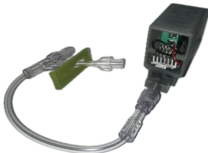
Figure 6. Final prototype of housing, cartridge, and circuit with connection to Luer lock shown.
