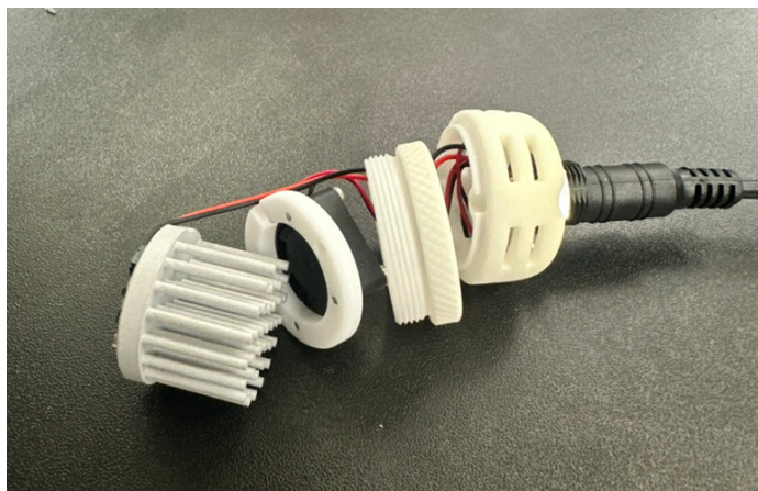
Figure 1. Disassembled mini-UV unit from AquiSense. Components from left to right are UV light attached to heat sink, fan, and connection to power supply.
