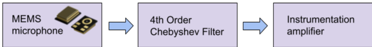
Figure 1: Block diagram of ultrasonic sensor
