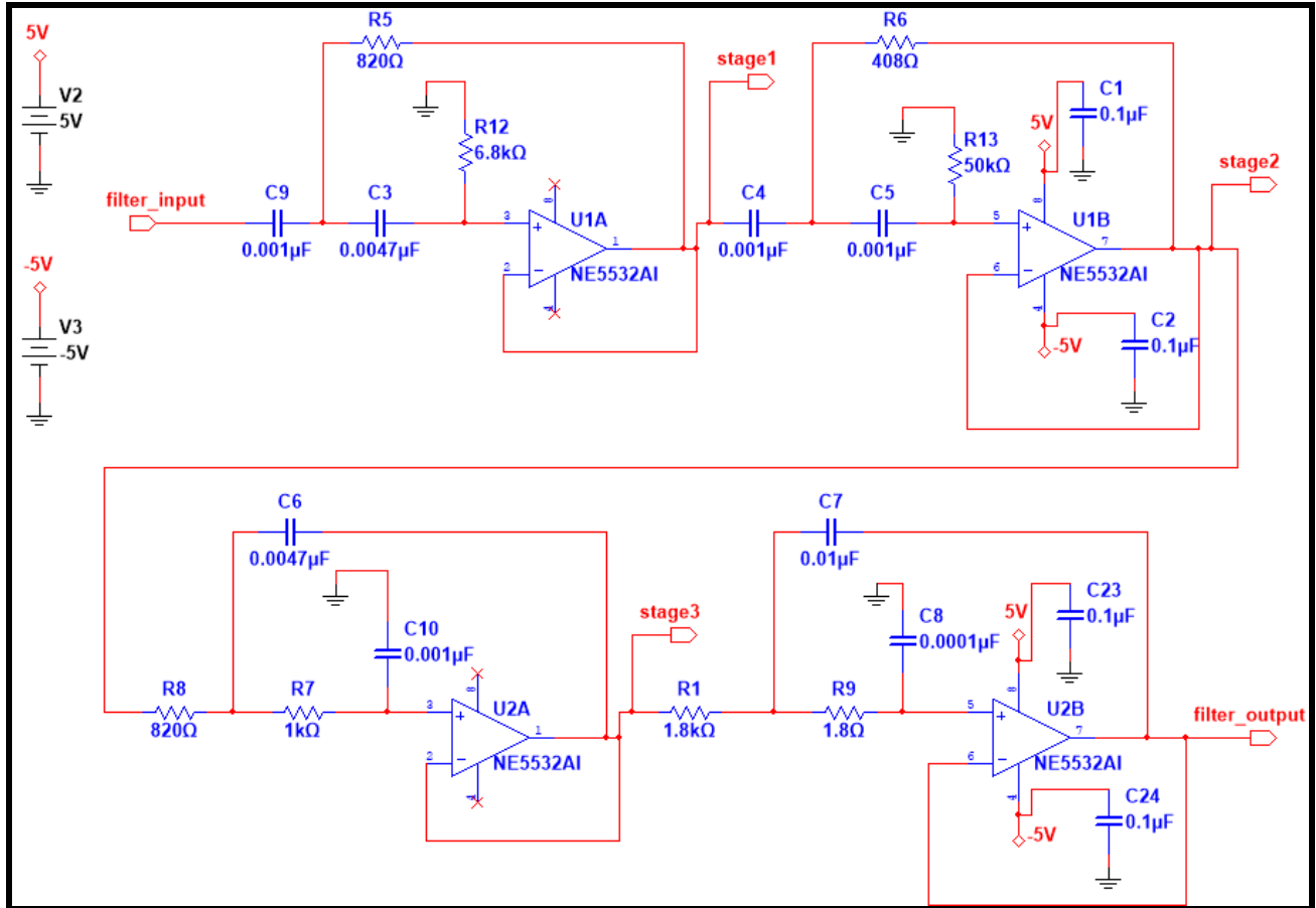
Figure 2: Filter Design
