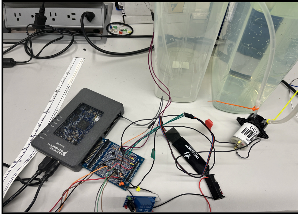
Figure 15: Breakout board
