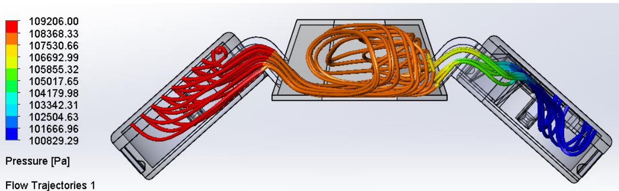
Figure 30: Top view of flow simulation displaying airflow trajectories and pressure values within system
