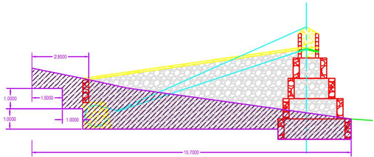
Left Abutment: Elevation
