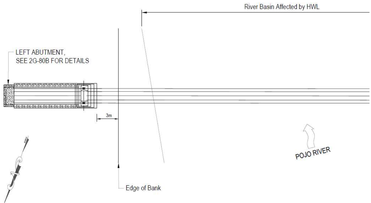
Figure 7: Plan view of left abutment
