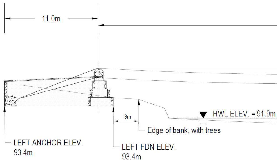
Figure 5: Elevation view of left abutment
