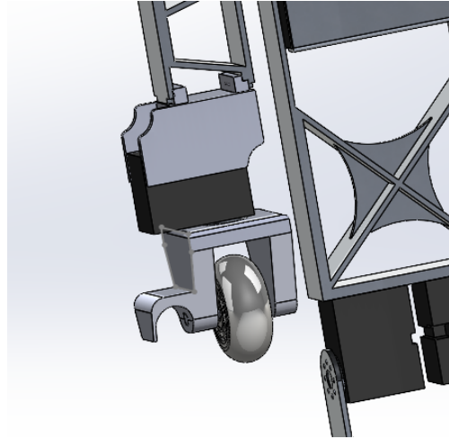
Figure 7: Compliant Hand/Wheel Final Design
