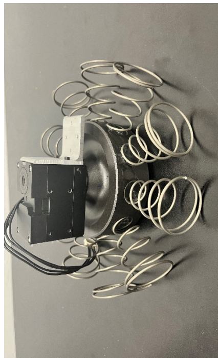
Figure 13: Image of the Completed Foot/Wheel Mechanism
