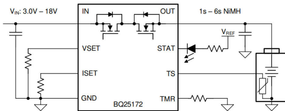
Figure 8-1. BQ25172 Simple Schematic
