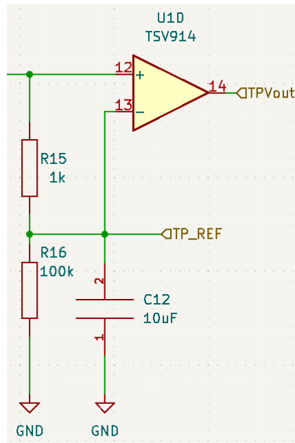
Figure 99 - Comparator Circuit
