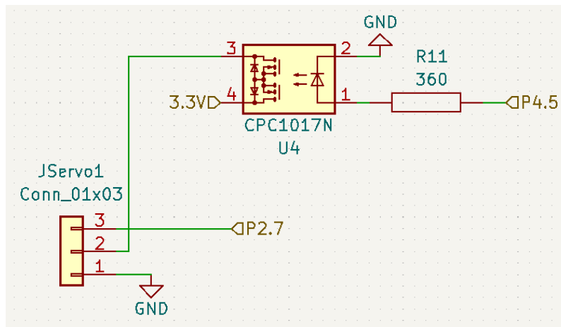
Figure 1515 - Servo [6] Driver with Solid-State Relay [8]
