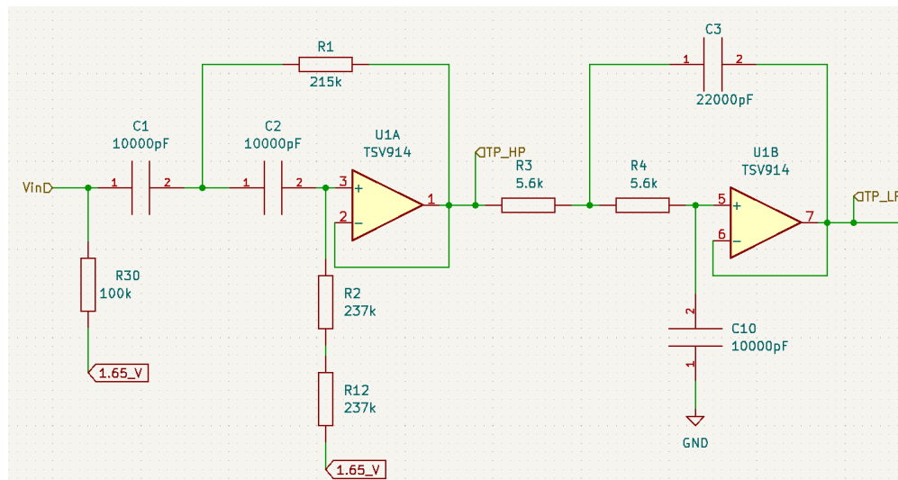
Figure 77 - Bandpass Filter
