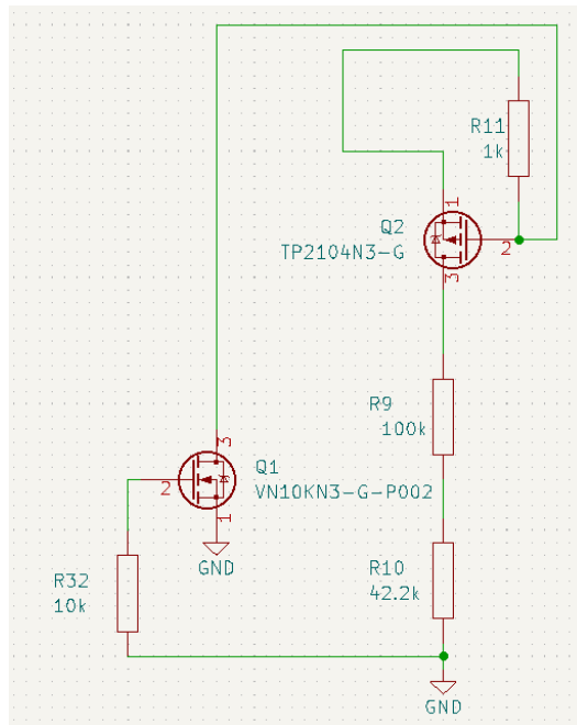
Figure 1313 - BJT Driven Resistive Divider for Battery Monitoring Prototype
