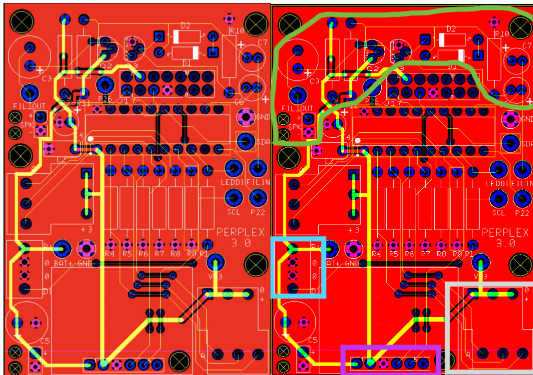
Figure 7. PCB Layout IMU:Purple, ADC:Gray, LED:Blue, Speaker:Green
