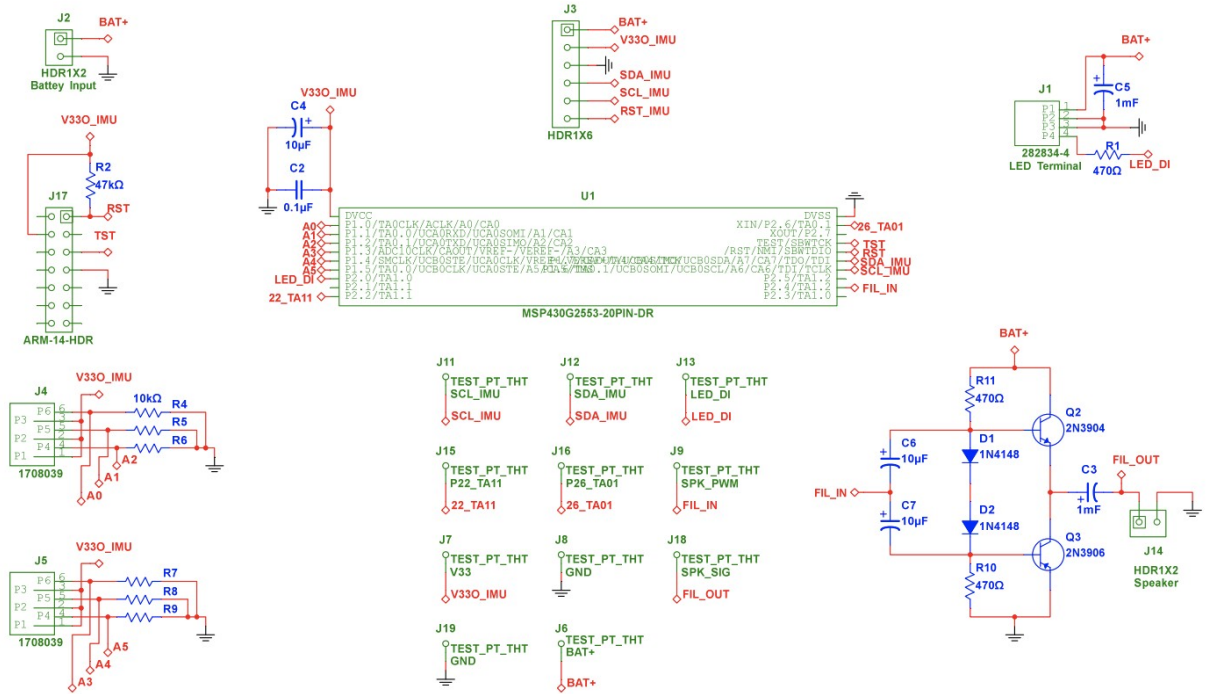
Figure 6. Multisim schematic
