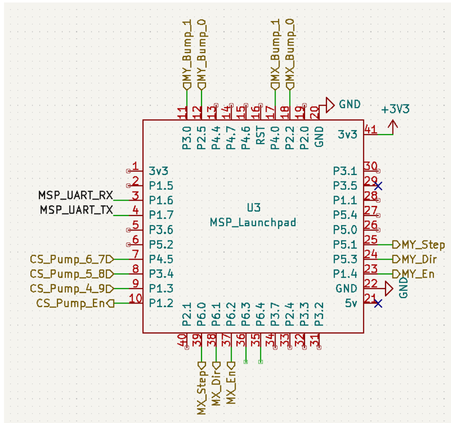
Figure 18: Microcontroller Pinout
