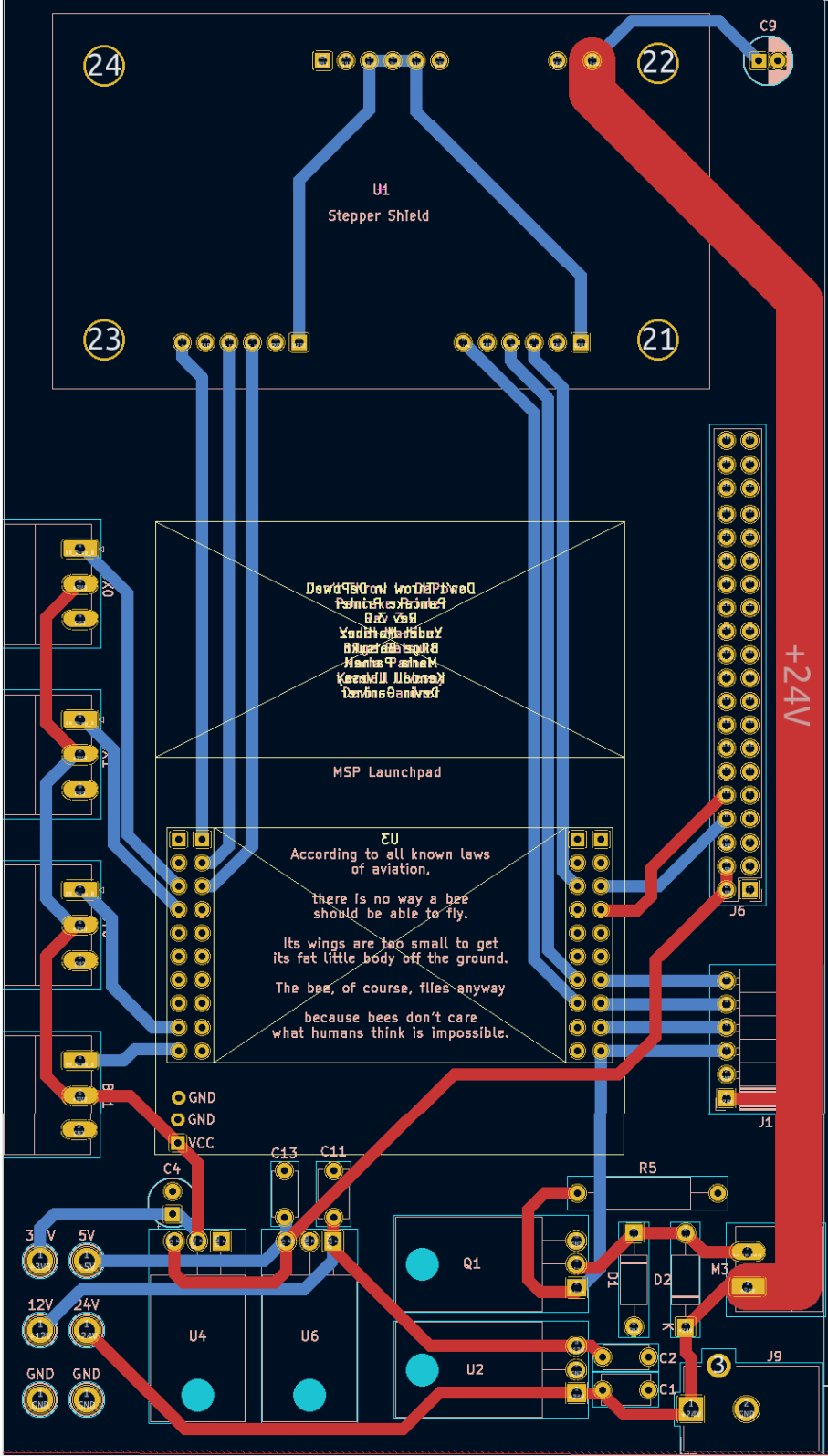
Figure 21: PCB Layout
