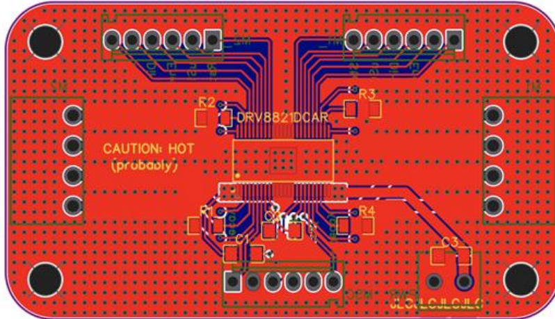
Figure 11: DRV8821 Breakout Board PCB
