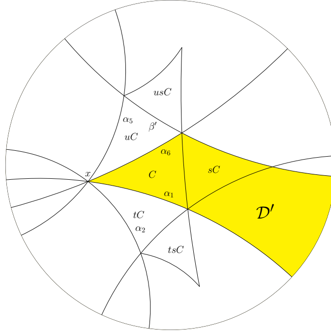
Figure 6.1: The roots \alpha_1, \alpha_6, \beta' with the region \mathcal{D}' in yellow.
