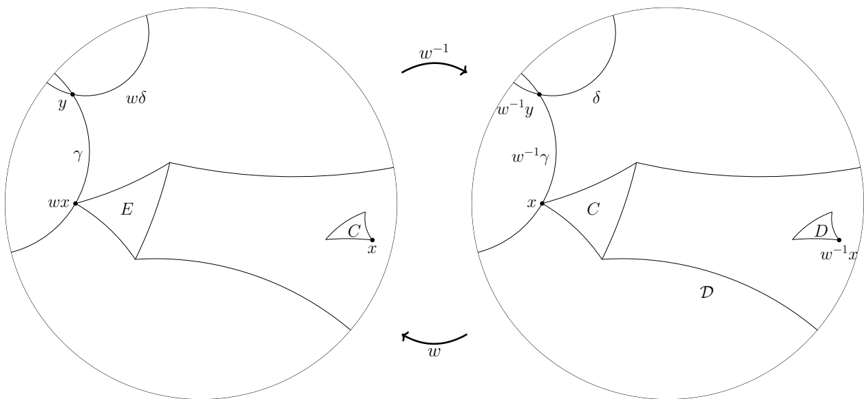
Figure 5.3: The effect of w and w^{-1} on the chambers and roots.
