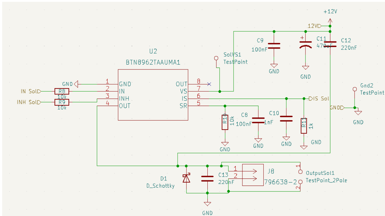
Figure 12: Solenoid Driver Schematic
