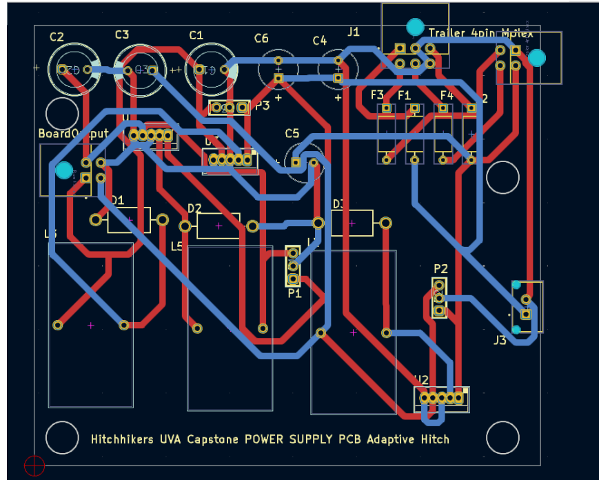
Figure 7: 'Power' PCB board layout
