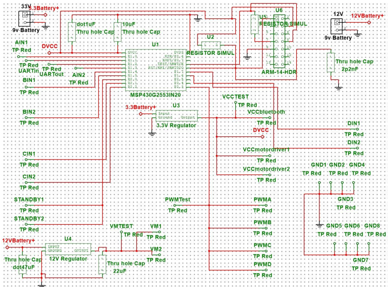
Figure 6 Multisim Schematic
