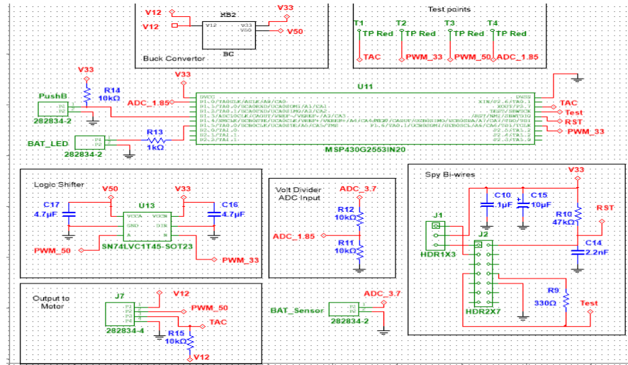
Figure 4: MSP430 Circuit Schematic
