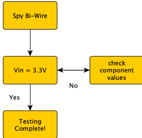
Figure 19: Spy Bi-Wire Test Plan
