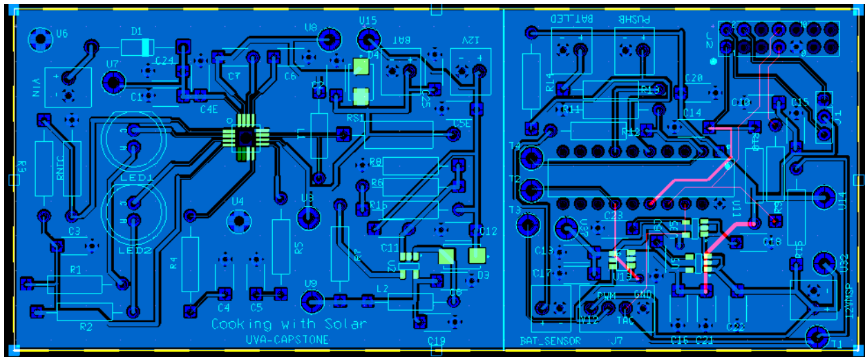
Figure 6: Ultiboard PCB
