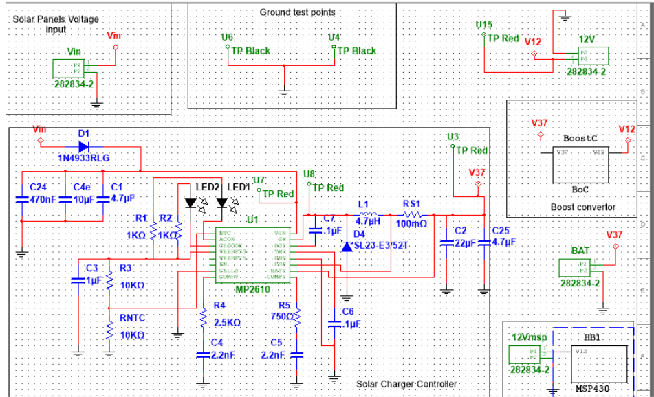
Figure 2: Power Management Schematic
