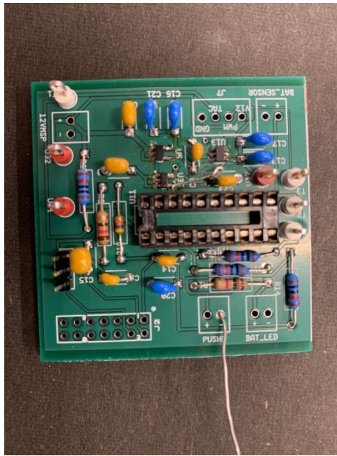
Figure 9: Soldered MSP430 PCB
