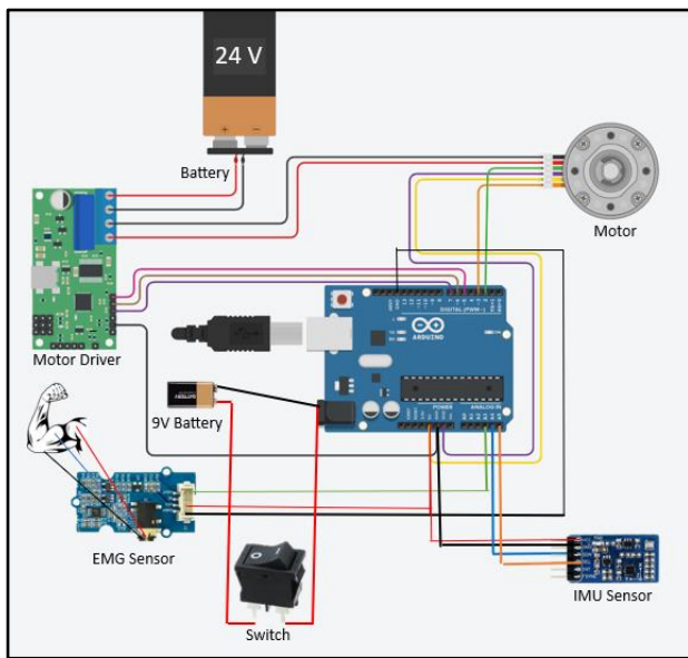
Fig 28. Circuit diagram of the final design
