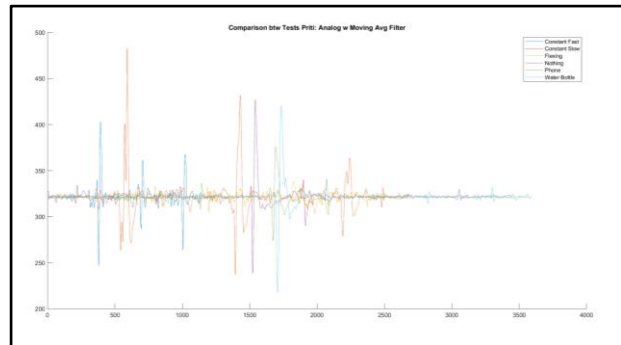
Fig 17. EMG data showing all series of tests conducted to characterize patterns; constant motion fast, constant motion slow, flexing, stop and start motion holding nothing, a phone, and a water bottle
