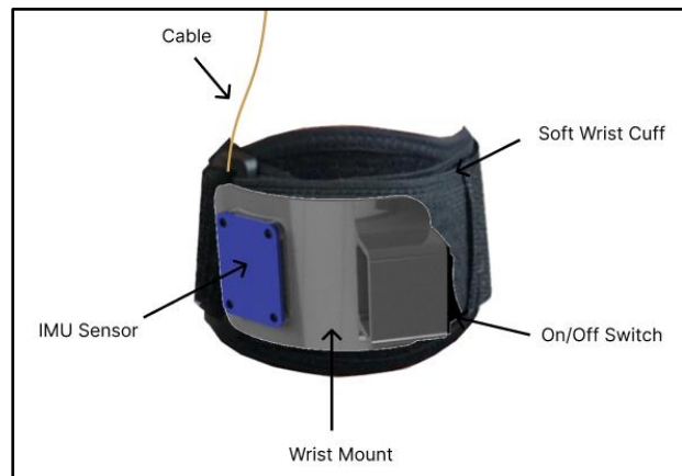
Fig 26. Wrist assembly
