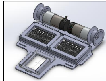
Fig 10. Electronic back mount design
