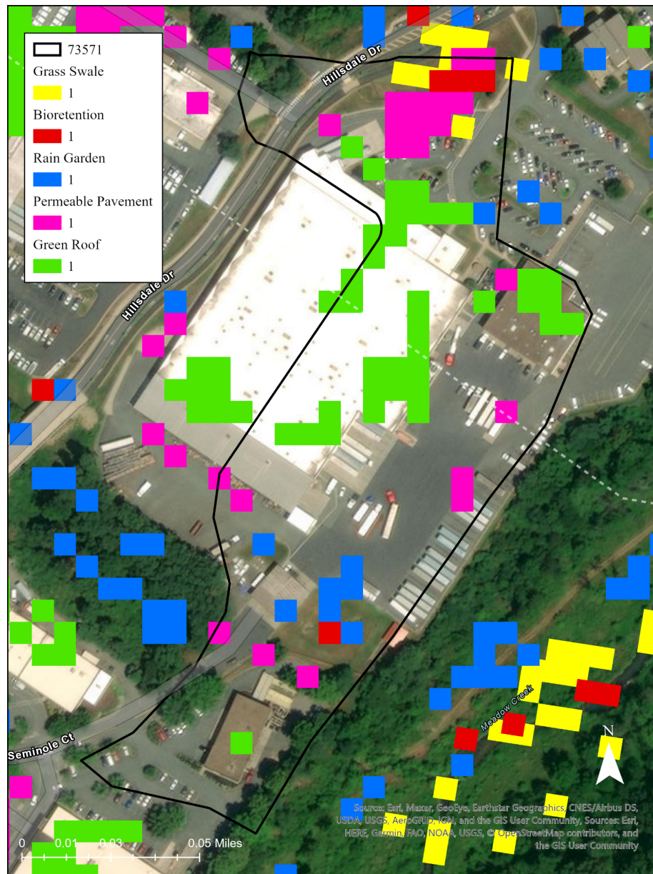
Figure 17. GI feasibility layers for subbasin 73571.
