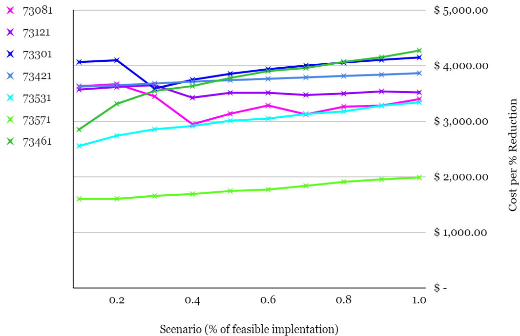
Figure 11. Cost per % reduction ($) versus PySWMM scenario (% of feasible implementation).
