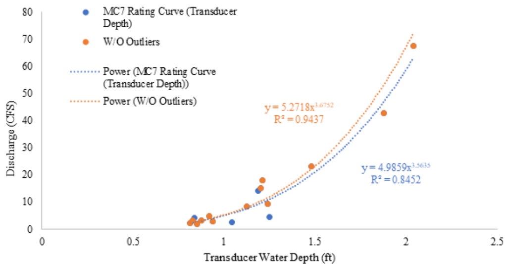
Figure 5. Rating curve produced for station MC 7 using results of fieldwork.
