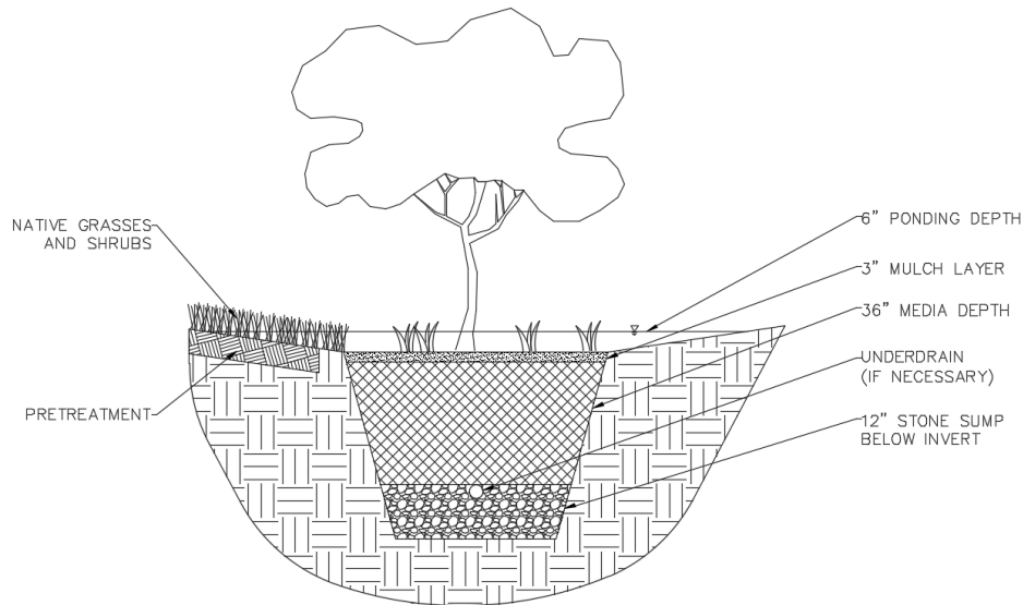
Figure 20. Section view of bioretention design.
