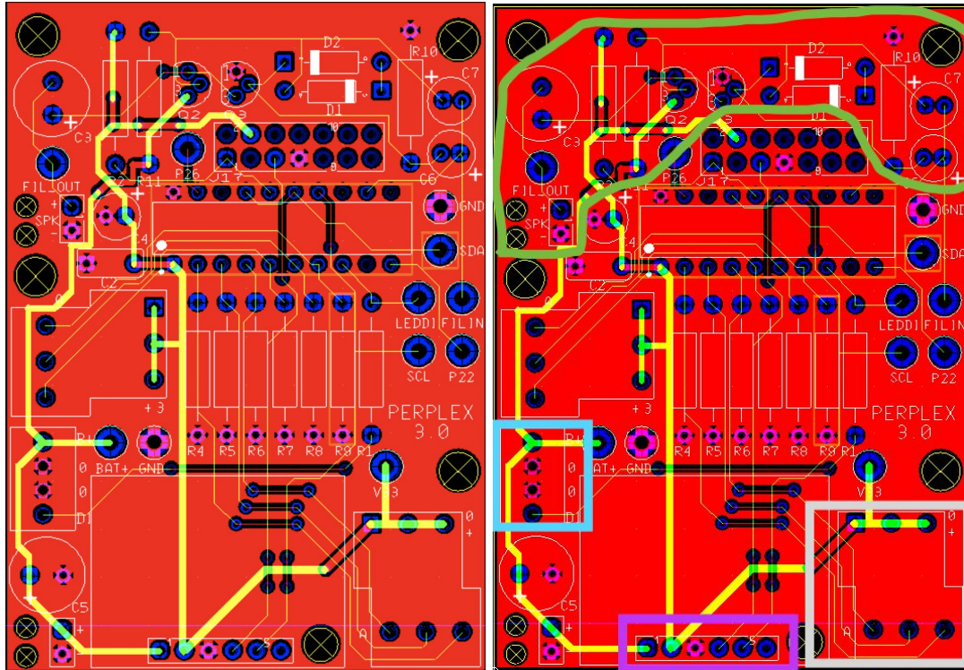
Figure 7. PCB Layout
