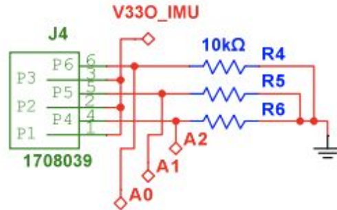
Figure 6.2. ADC input
