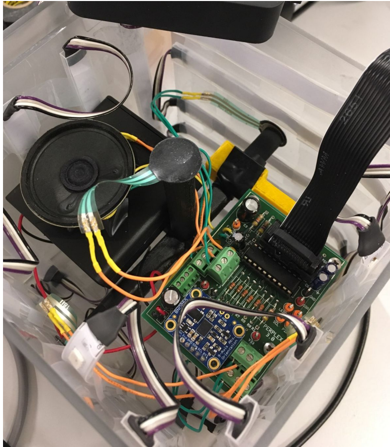
Figure 2. Cubetrix internals
