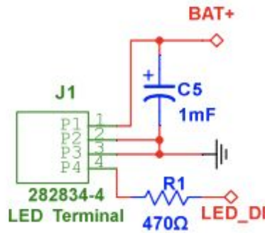
Figure 6.3. LED connection
