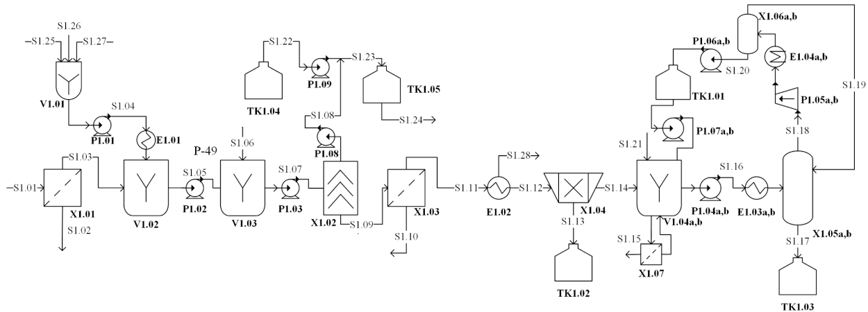
Figure 3.2.1 Process flow diagram for the seed oil extraction block
