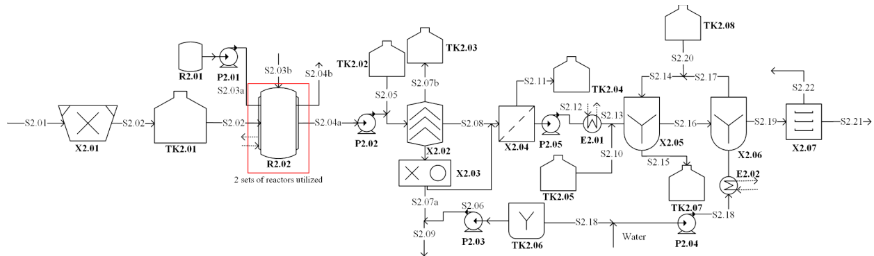
Figure 3.3.1 Process flow diagram for sesame cake fermentation
