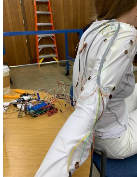
Fig. 9. The textile version of the sensor array depicts the snap connectors to gel electrodes, rainbow wire cables, sensor array, and wire-to-fabric stabilizing glue and tape
