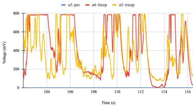
Bicep Curl - Upper Arm EMG Sensor Data
