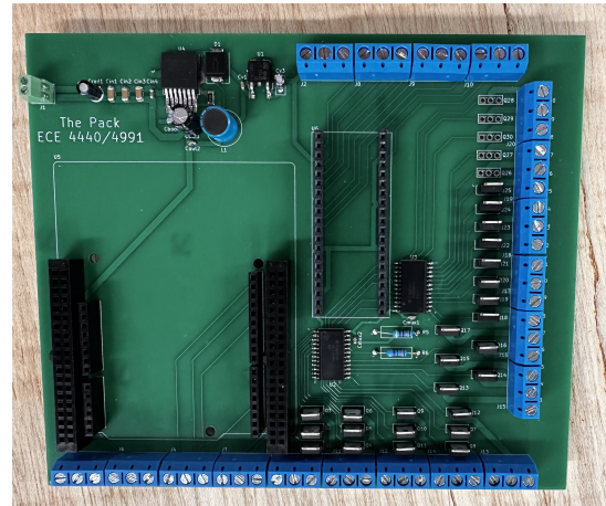
Fig. 7. Control Board for the LED Matrix
